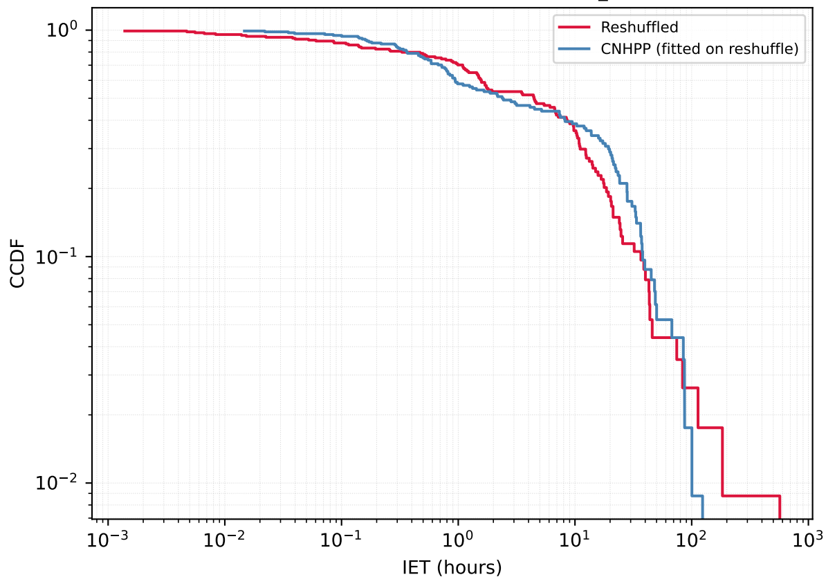
User 1753465784 - Reshuffled vs CNHPP A_{\text{fit}}=0.3543
